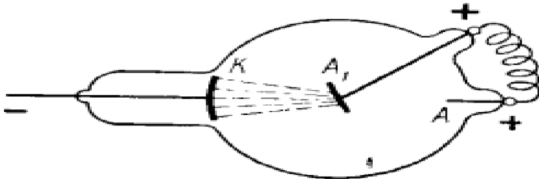
Fig. 1. Diagram of an ion x-ray tube. A - anode; A; - anticathode; K-cathode.
